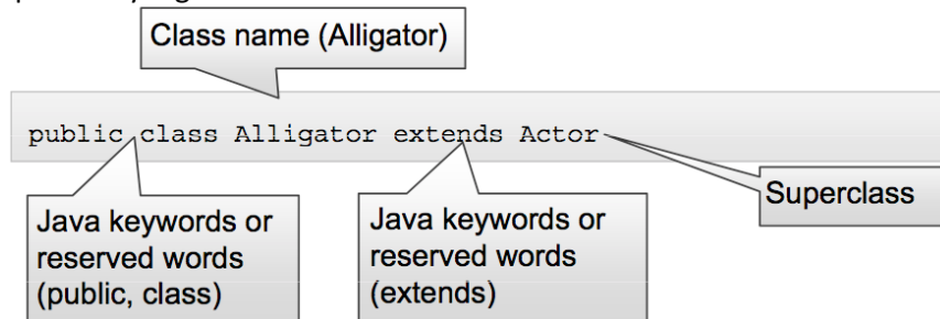
Gambar 23 Class Definition
