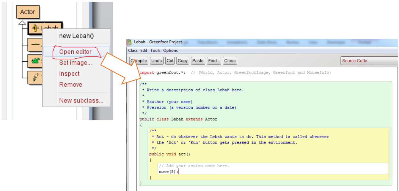
Gambar 21 Source code
