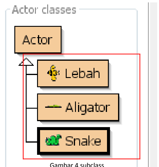
Gambar 4 subclass
