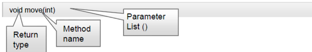
Gambar 7 contoh method
